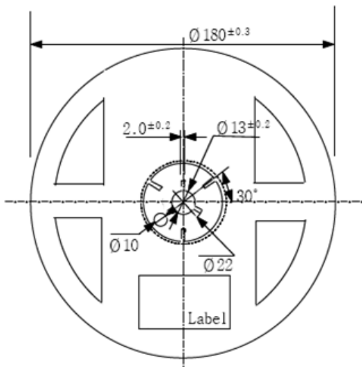
REEL DIAGRAM
