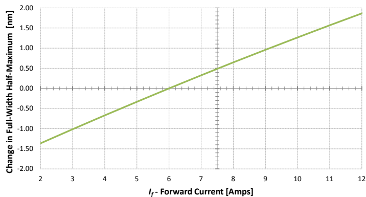
Change in Full-Width Half-Maximum vs Forward Current ( I_f ) Referenced to 6 A and T_j = 120^\circ\text{C}
