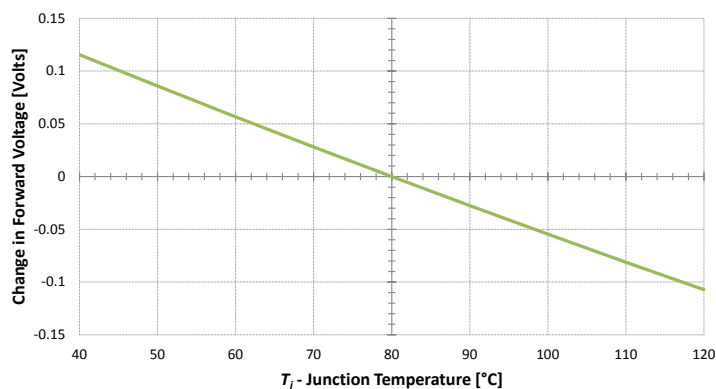
Change in Forward Voltage ( V_f ) vs Junction Temperature ( T_j ) Referenced to 80^\circ\text{C}
