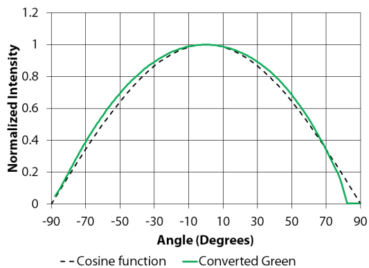
Angular Intensity Distribution (Typical)
