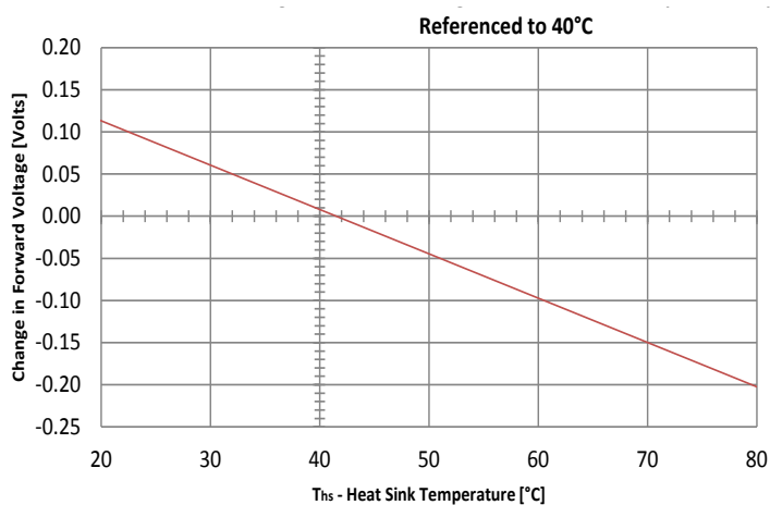
Forward Voltage vs Heat Sink Temperature
