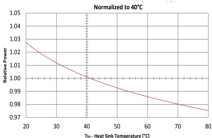
Relative Power vs Heat Sink Temperature
