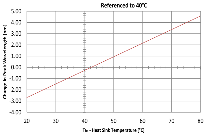
Peak Wavelength vs Heat Sink Temperature
