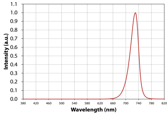
Typical Spectrum
