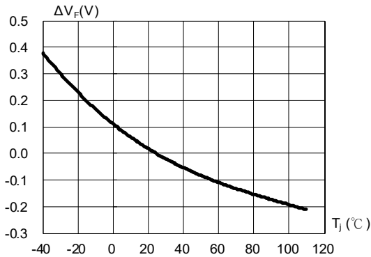
Fig. 3 Relative Forward Voltage vs. Junction Temperature \Delta V_F = V_F - V_F(25^\circ C) = f(T_J) ; I F = 50mA
