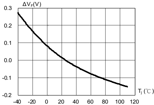
Fig. 3 Relative Forward Voltage vs. Junction Temperature \Delta V_F = V_F - V_F(25^\circ\text{C}) = f(T_J); I_F = 140\text{mA}
