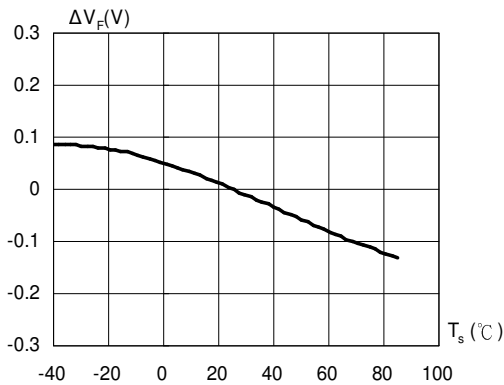
Fig.3 Relative Forward Voltage vs. Solder Point Temperature \Delta V_F = V_F - V_F(25^\circ\text{C}) = f(T_s) ; I F = 20mA
