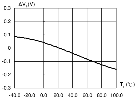
Fig.3 Relative Forward Voltage vs. Solder Point Temperature \Delta V_F = V_F - V_{F(25^\circ C)} = f(T_s) ; I F = 10mA
