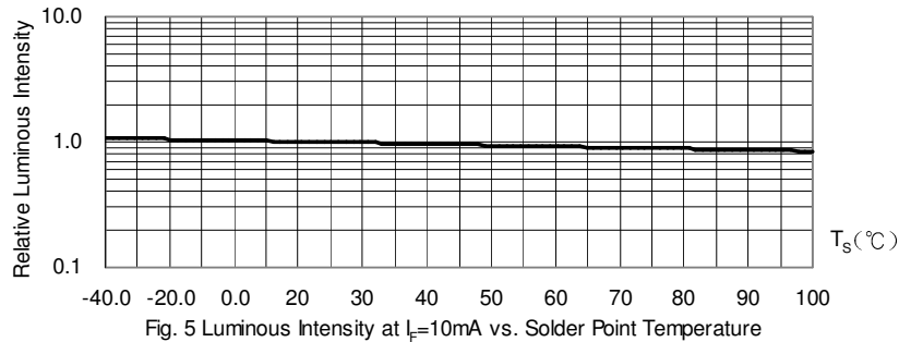
Fig.5 Luminous Intensity at I F =10mA vs. Solder Point Temperature
