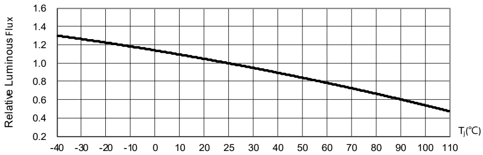
Fig. 5 Luminous Flux at I=50mA vs. Junction Temperature
