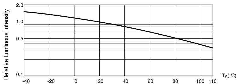
Fig. 5 Luminous Intensity at I_F = 20mA vs. Solder Point Temperature
