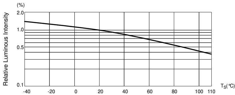
Fig. 5 Luminous Intensity at I_F = 50mA vs. Solder Point Temperature
