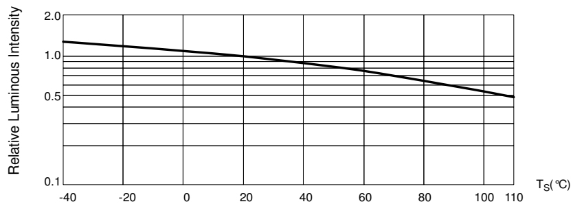
Fig. 5 Luminous Intensity at I_F = 20\text{mA} vs. Solder Point Temperature
