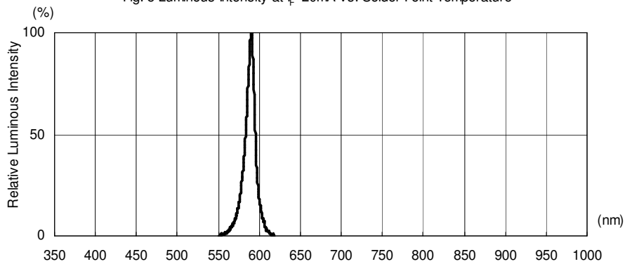
Fig.6. Relative Luminous Intensity vs. Wavelength
