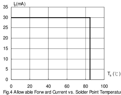
Fig.4 Allowable Forward Current vs. Solder Point Temperature
