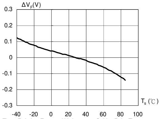
Fig.3 Relative Forward Voltage vs. Solder Point Temperature
