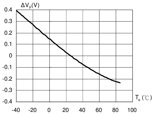
Fig. 3 Relative Forward Voltage vs. Solder Point Temperature \Delta V_F = V_F - V_F(25^\circ\text{C}) = f(T_s) ; I F = 20mA
