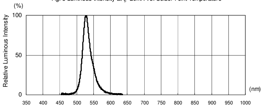
Fig 6. Relative Luminous Intensity vs. Wavelength
