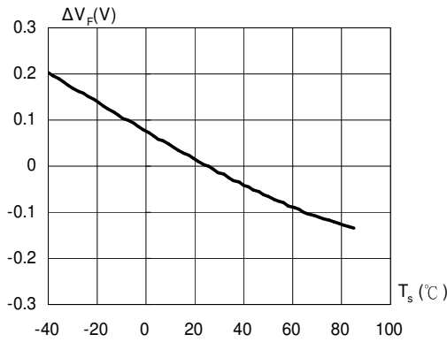
Fig.3 Relative Forward Voltage vs. Solder Point Temperature \Delta V_F = V_F - V_F(25^\circ\text{C}) = f(T_s); I_F = 20\text{mA}
