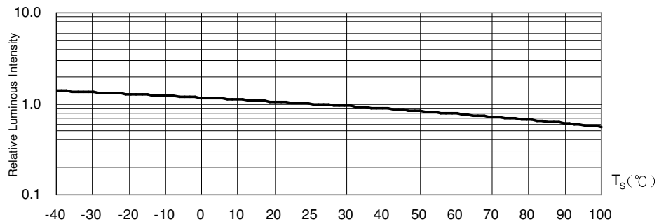
Fig.5 Luminous Intensity at I_F=20\text{mA} vs. Solder Point Temperature
