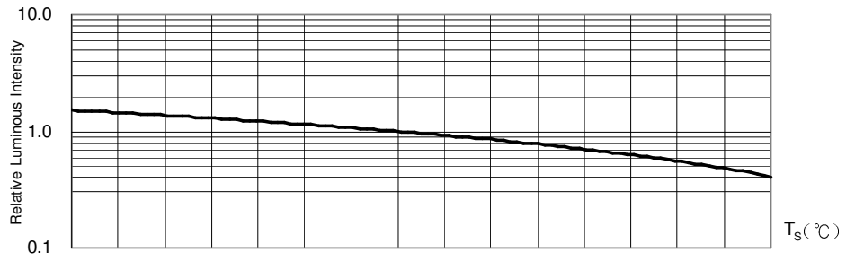
Fig. 5 Luminous Intensity at I F =20mA vs. Solder Point Temperature
