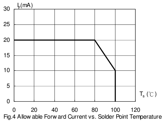
Fig.4 Allowable Forward Current vs. Solder Point Temperature
