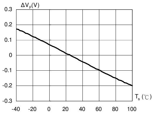
Fig. 3 Relative Forward Voltage vs. Solder Point Temperature \Delta V_F = V_F - V_F(25^\circ\text{C}) = f(T_s); I_F = 20\text{mA}
