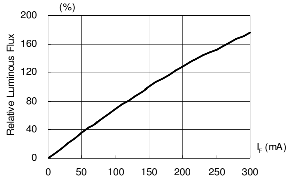
Fig.2 Luminous Flux vs. Forward Current
