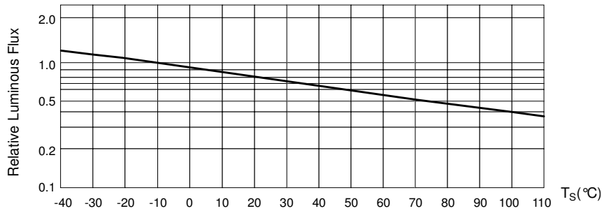
Fig. 5 Luminous Flux at I_F=350mA vs. Solder Point Temperature
