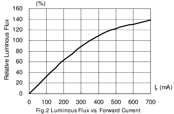
Fig.2 Luminous Flux vs. Forward Current
