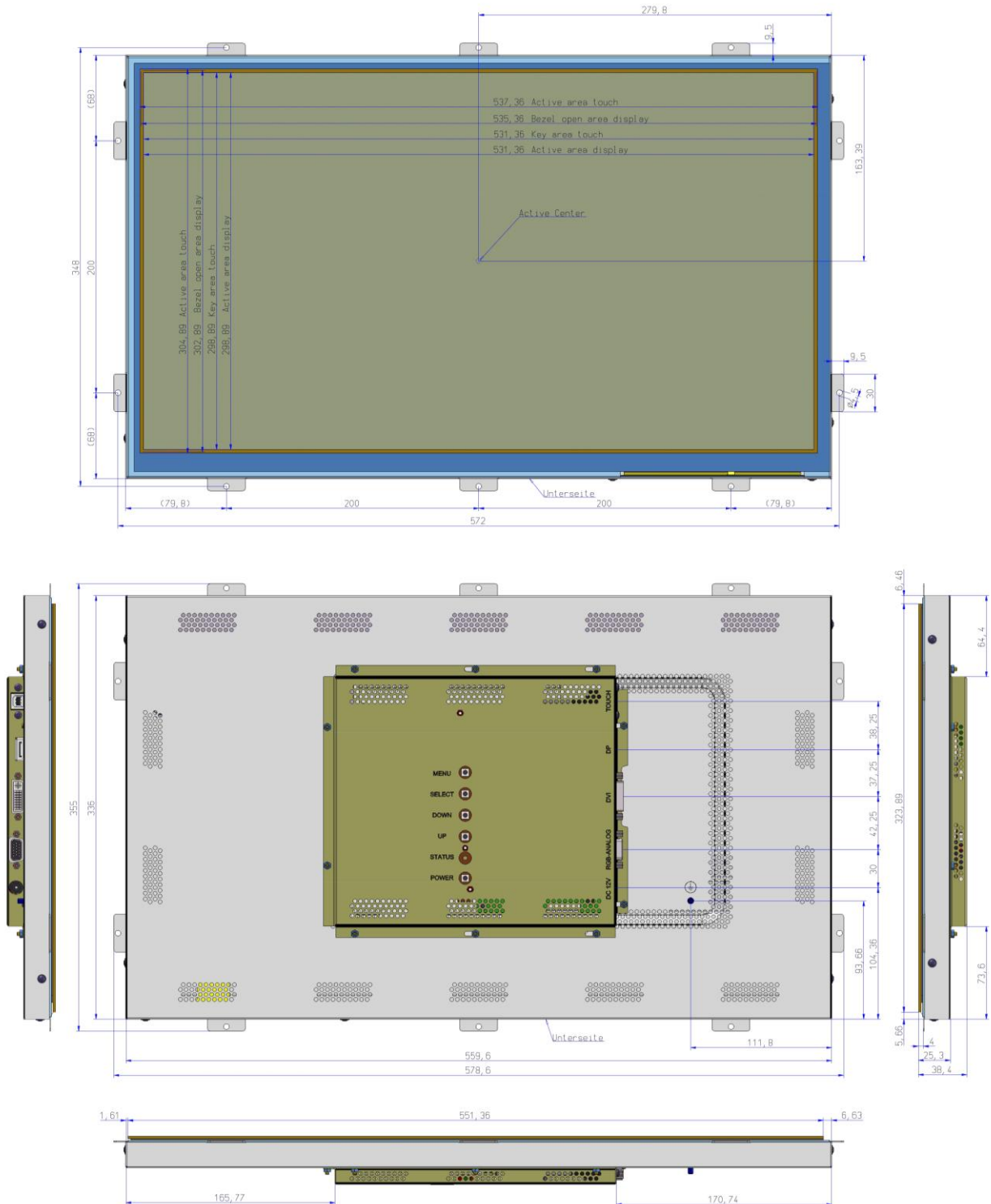
Figure 1: Mechanical Outlines
