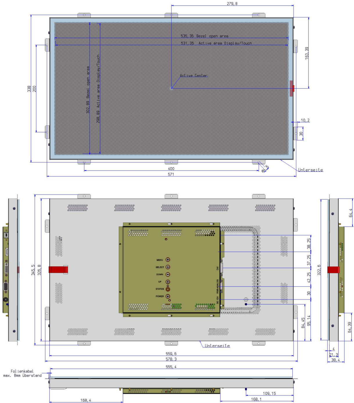
Figure 1: Mechanical Outlines
