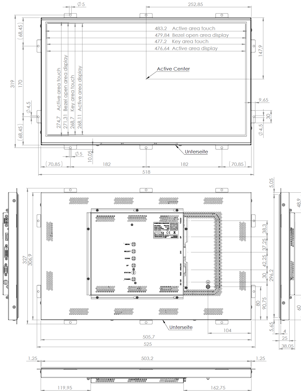
Figure 1: Mechanical Outlines
