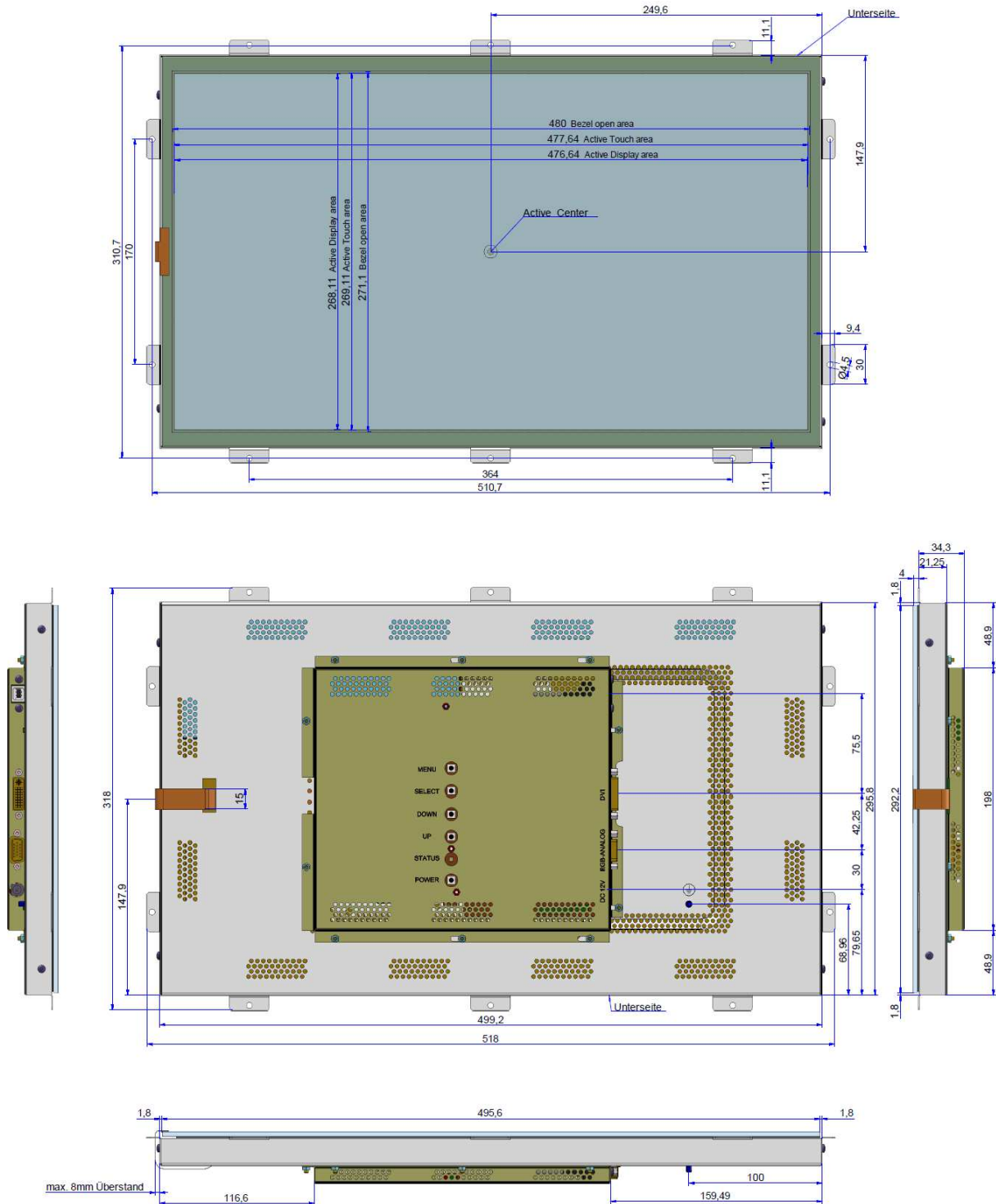
Figure 1: Mechanical Outlines
