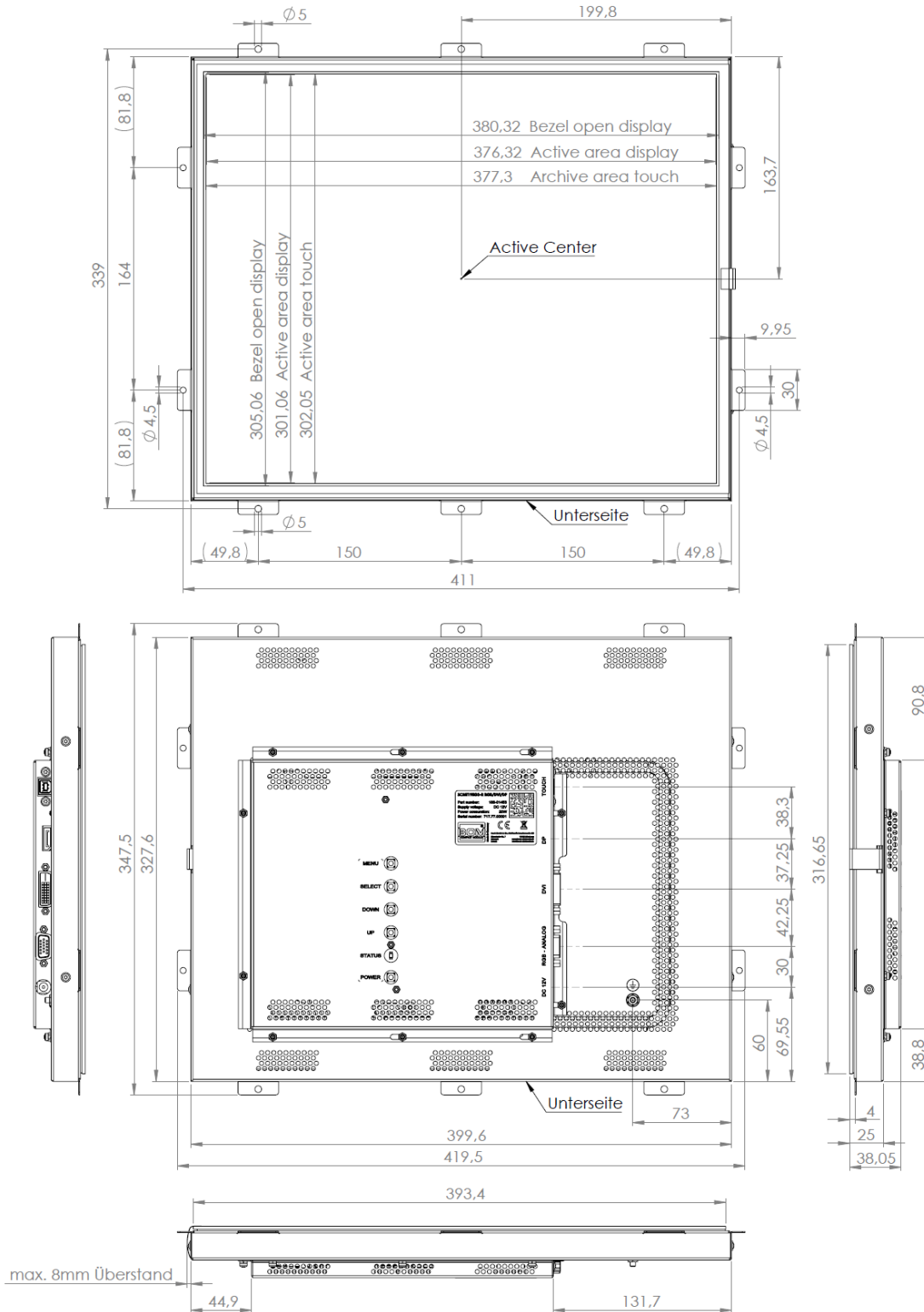
Figure 1: Mechanical Outlines
