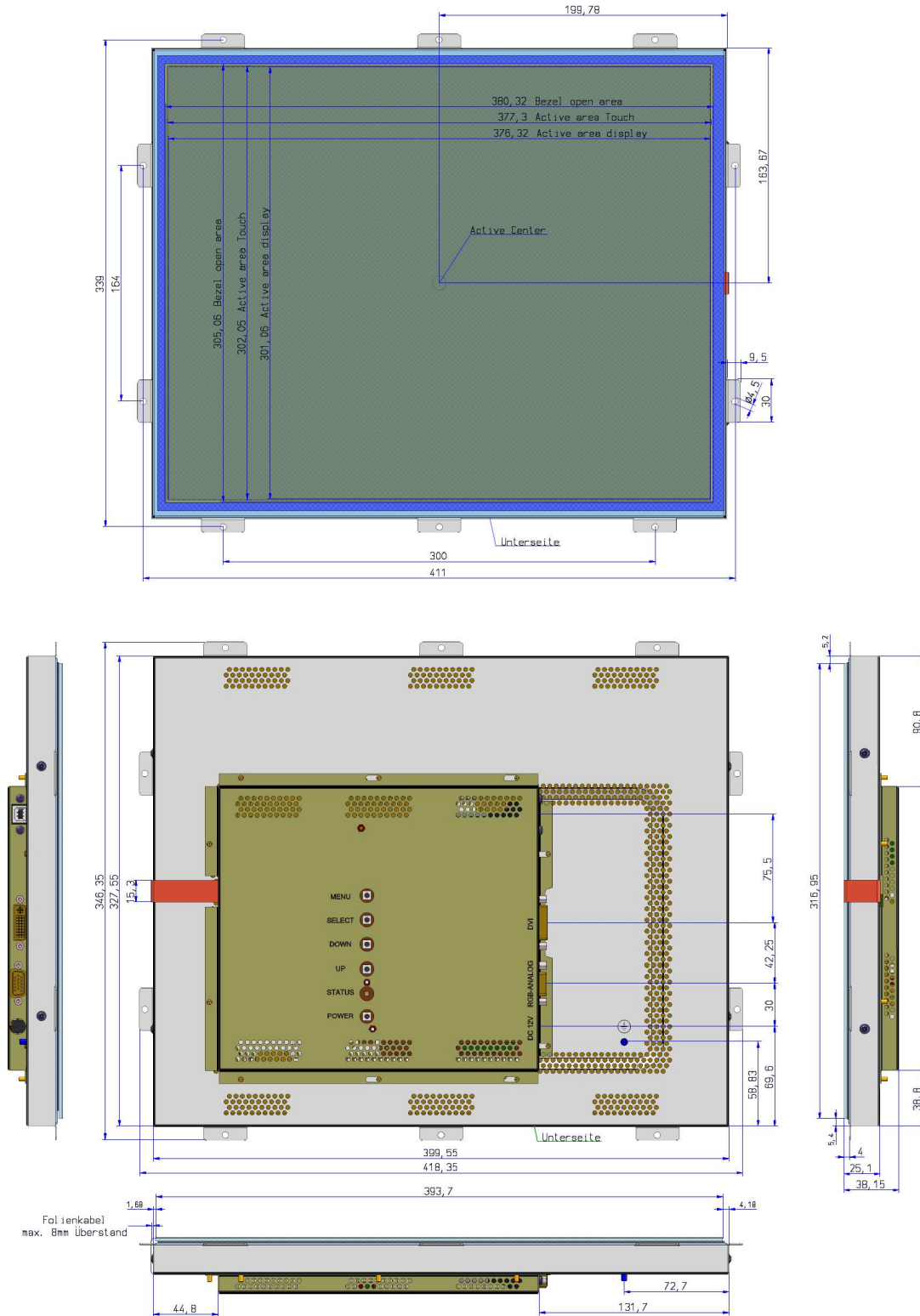
Figure 1: Mechanical Outlines
