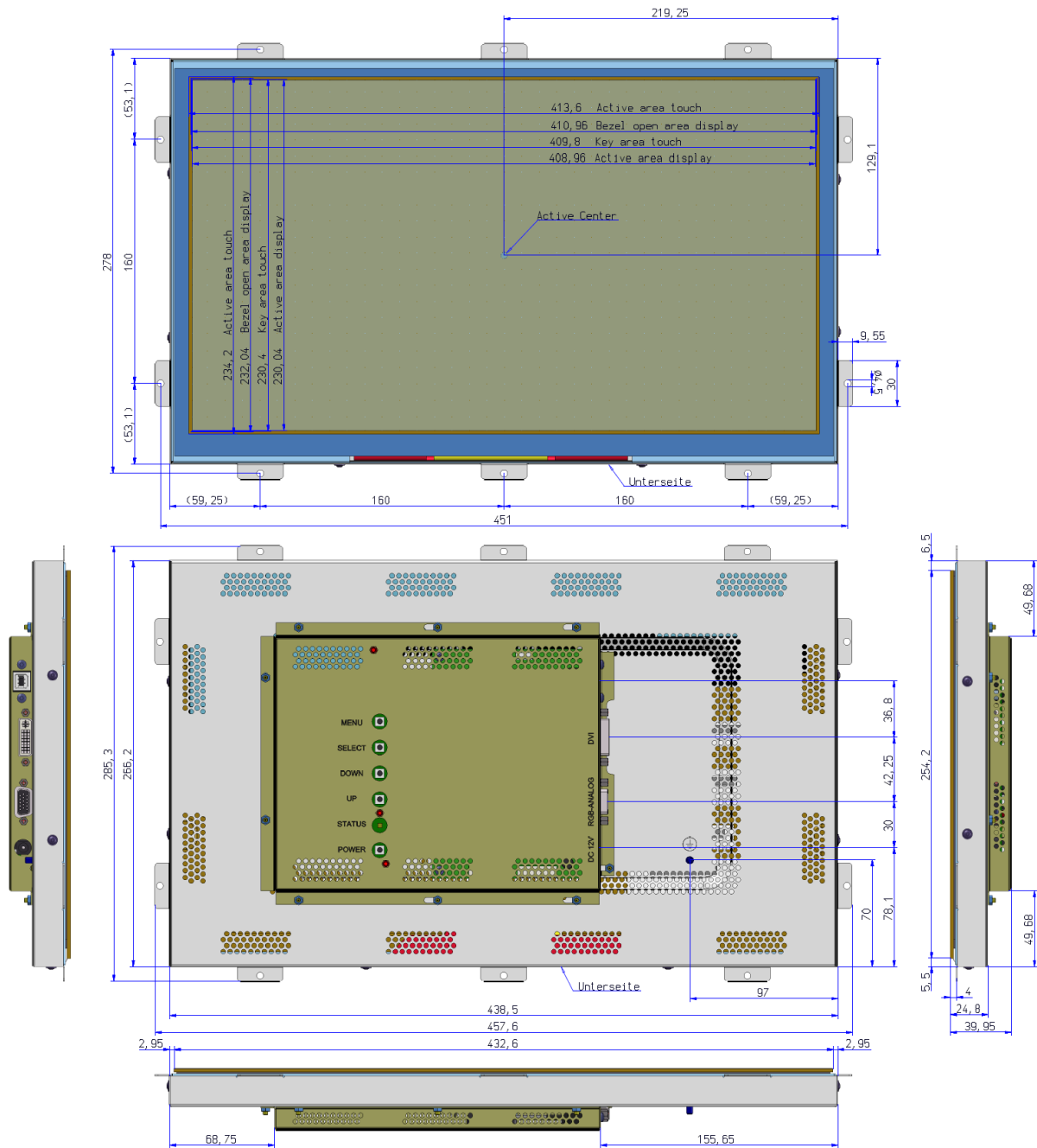
Figure 1: Mechanical Outlines
