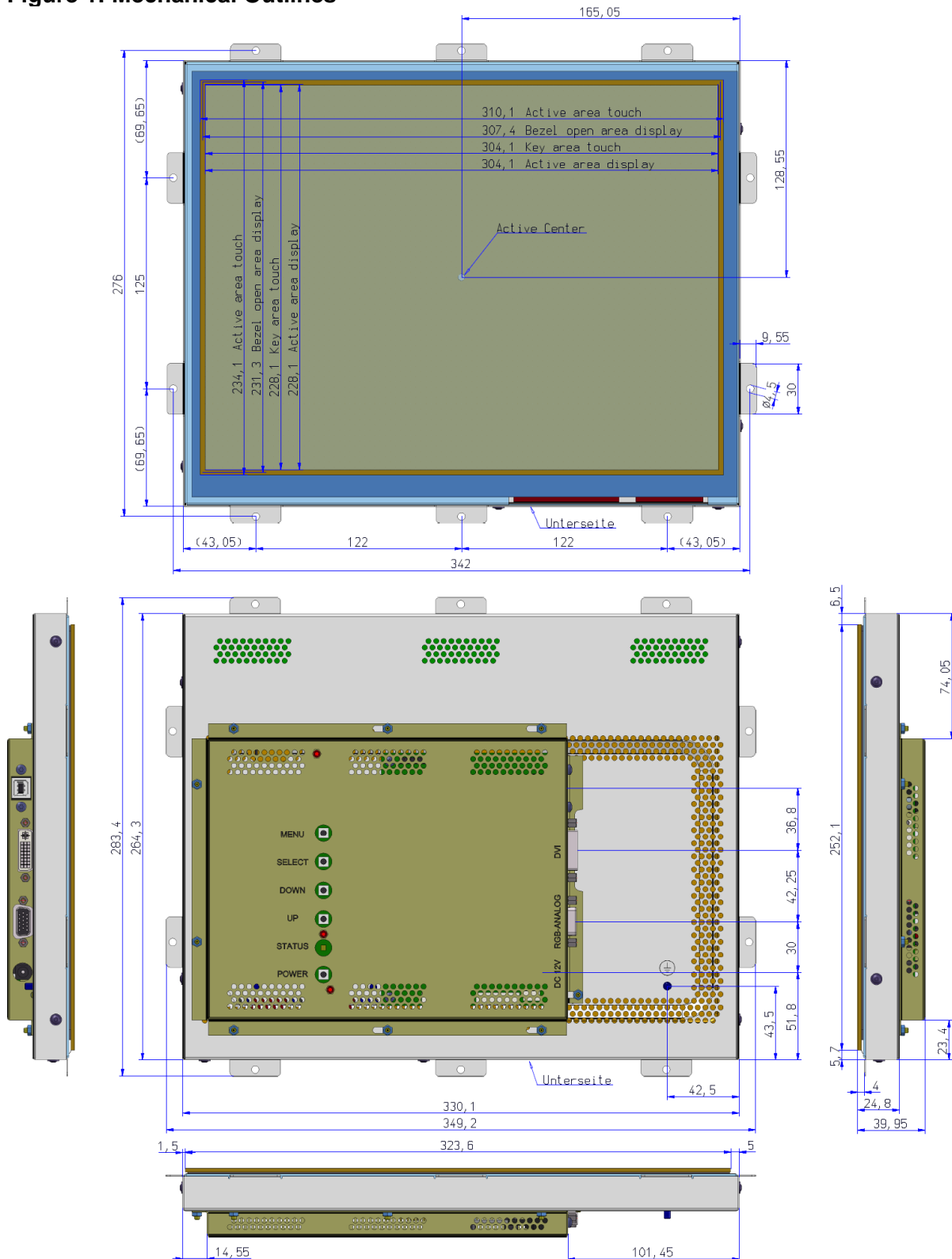
Figure 1: Mechanical Outlines
