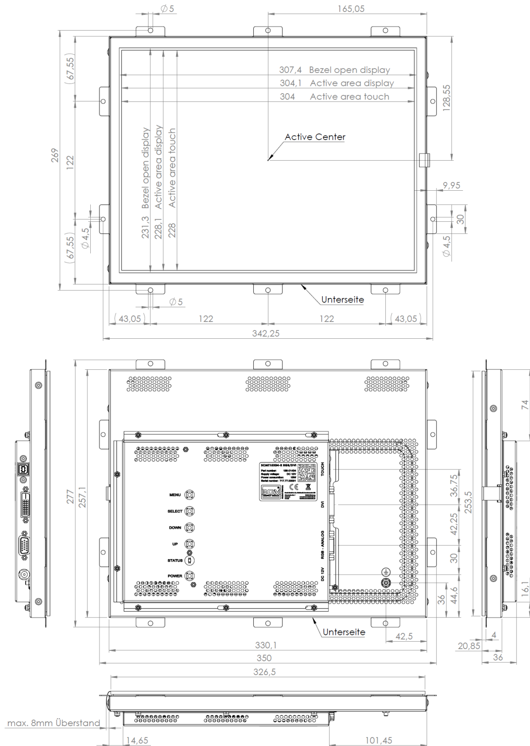
Figure 1: Mechanical Outlines
