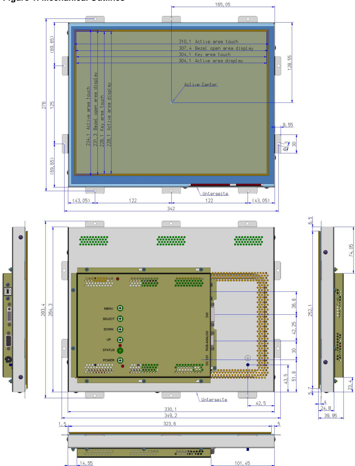
Figure 1: Mechanical Outlines
