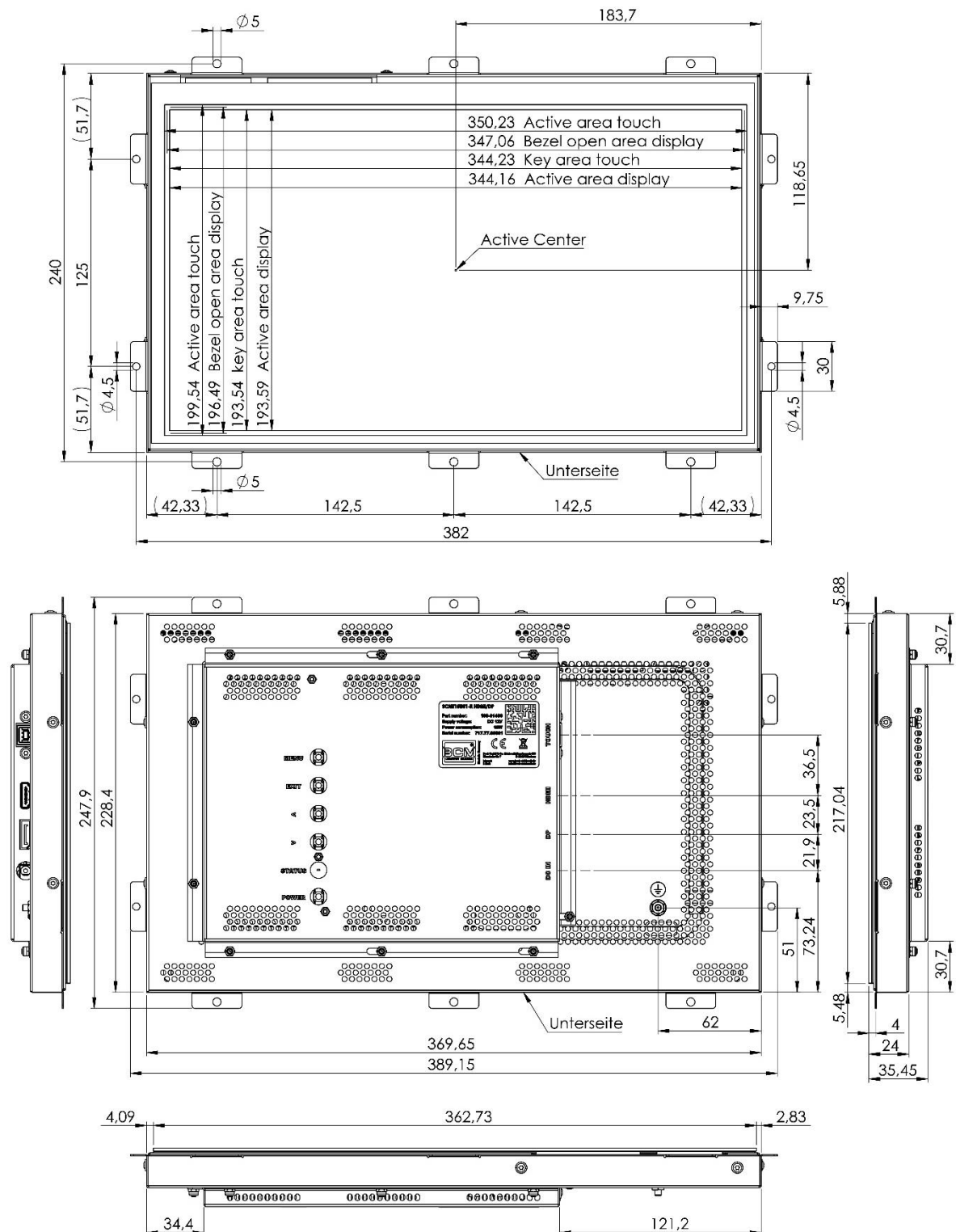
Figure 1: Mechanical Outlines
