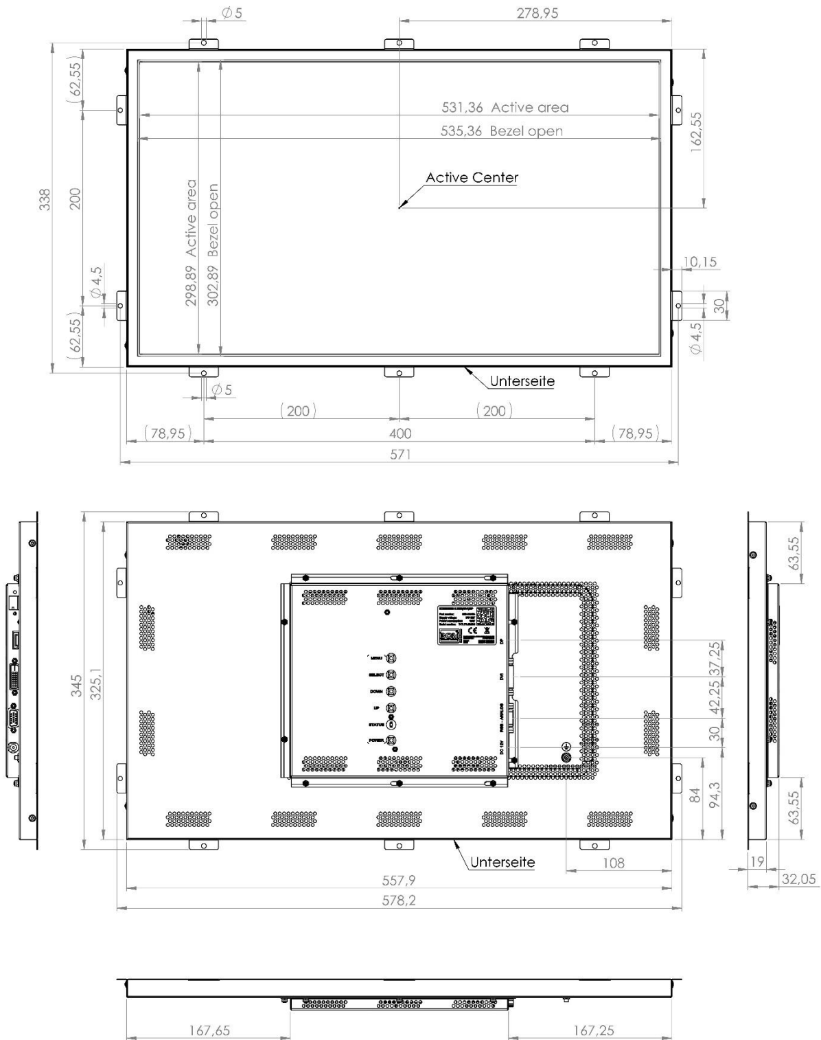
Figure 1: Mechanical Outlines
