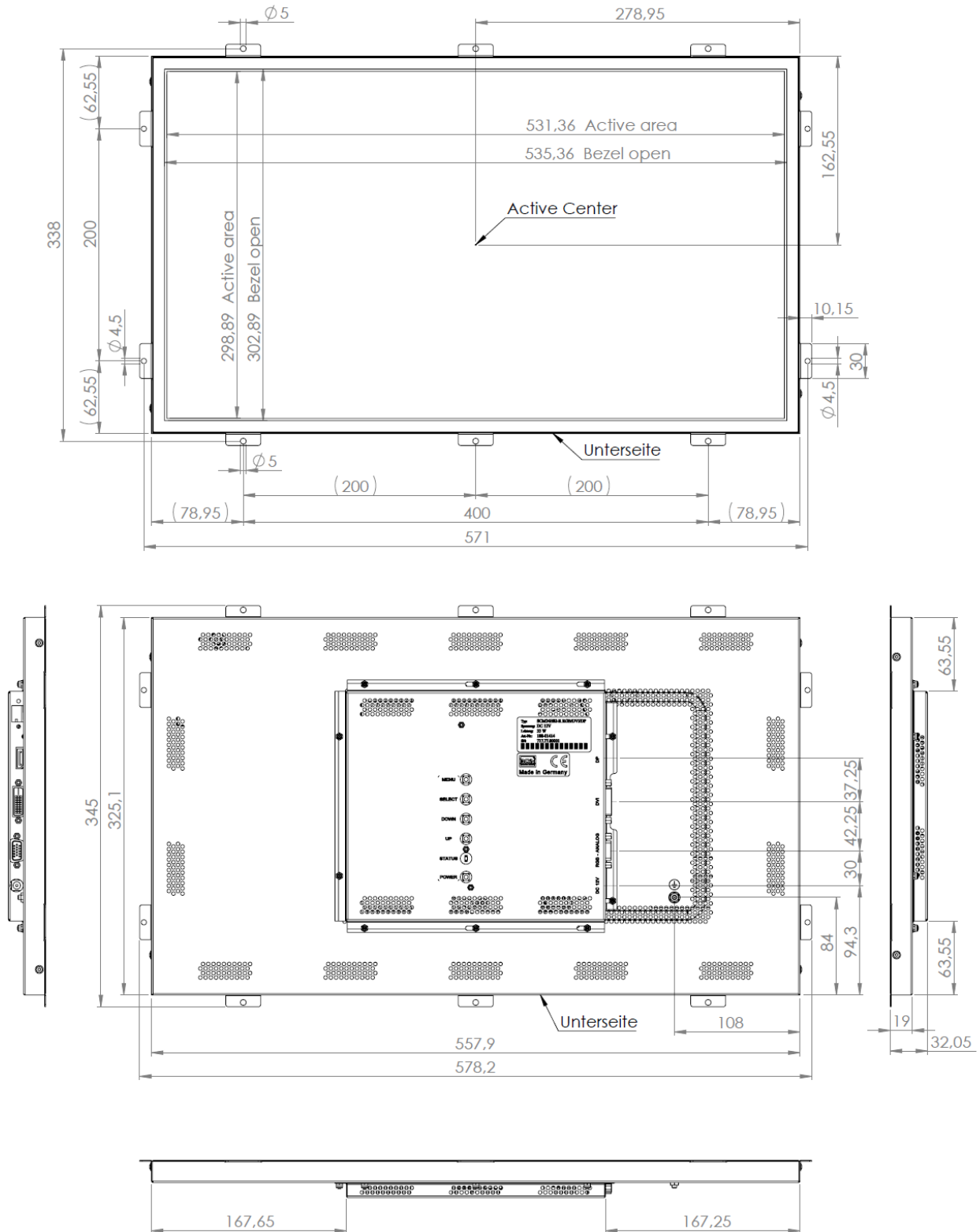
Figure 1: Mechanical Outlines
