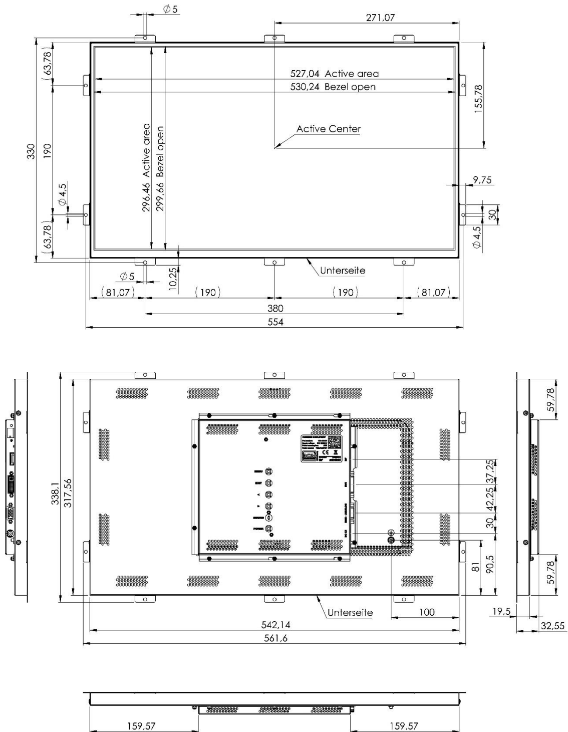
Figure 1: Mechanical Outlines
