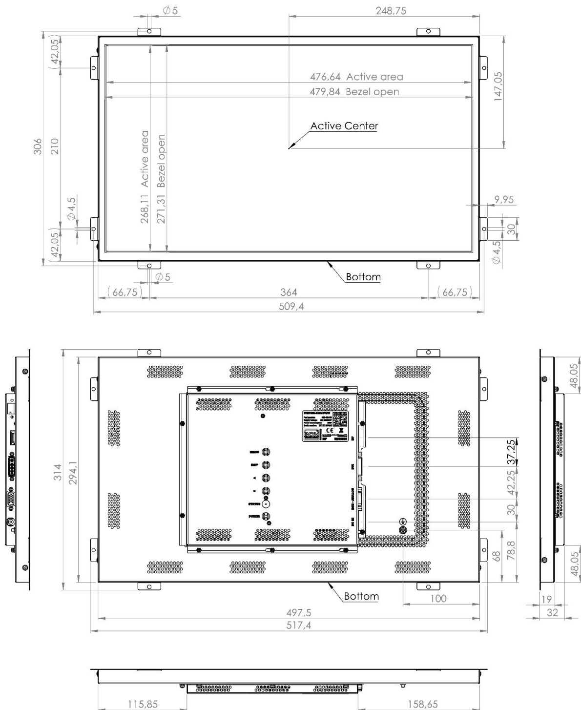
Figure 1: Mechanical Outlines
