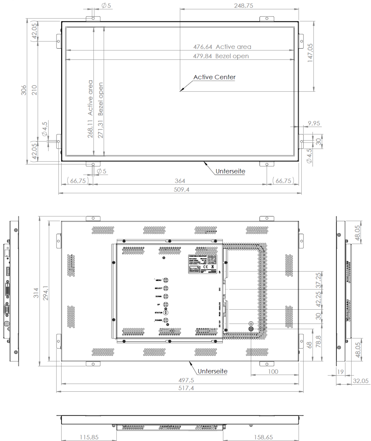
Figure 1: Mechanical Outlines
