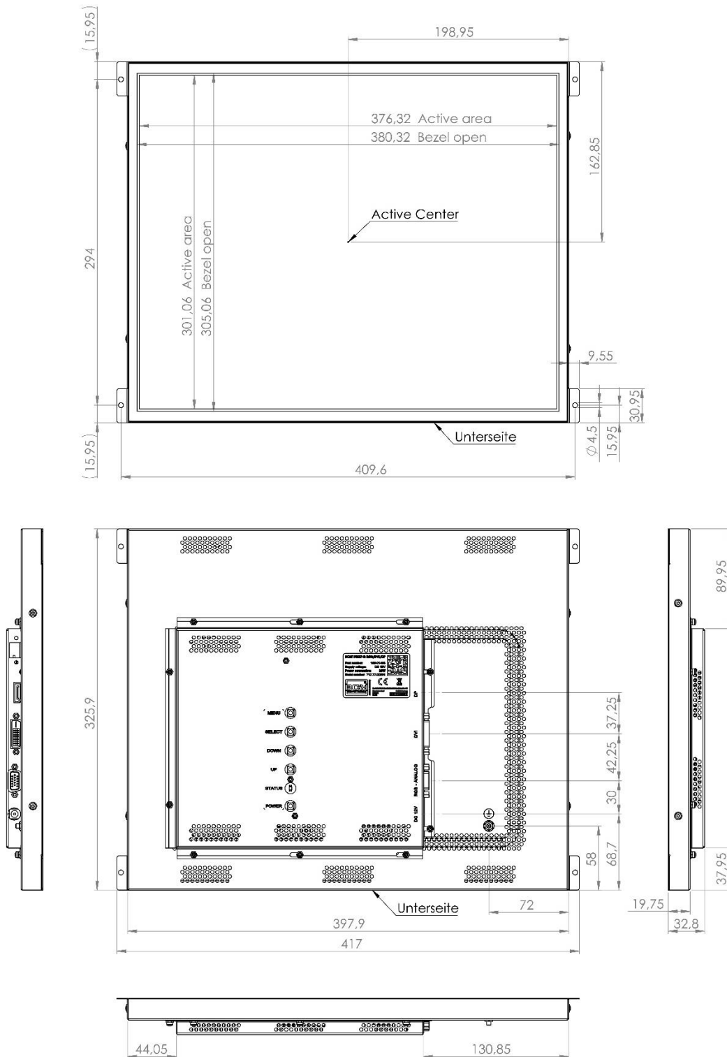
Figure 1: Mechanical Outlines
