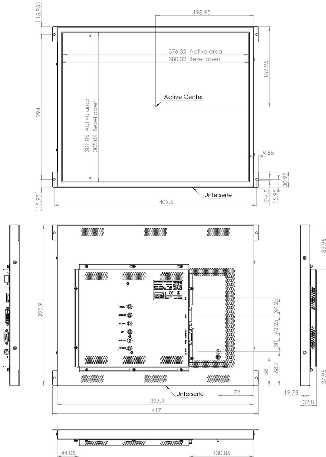
Figure 1: Mechanical Outlines
