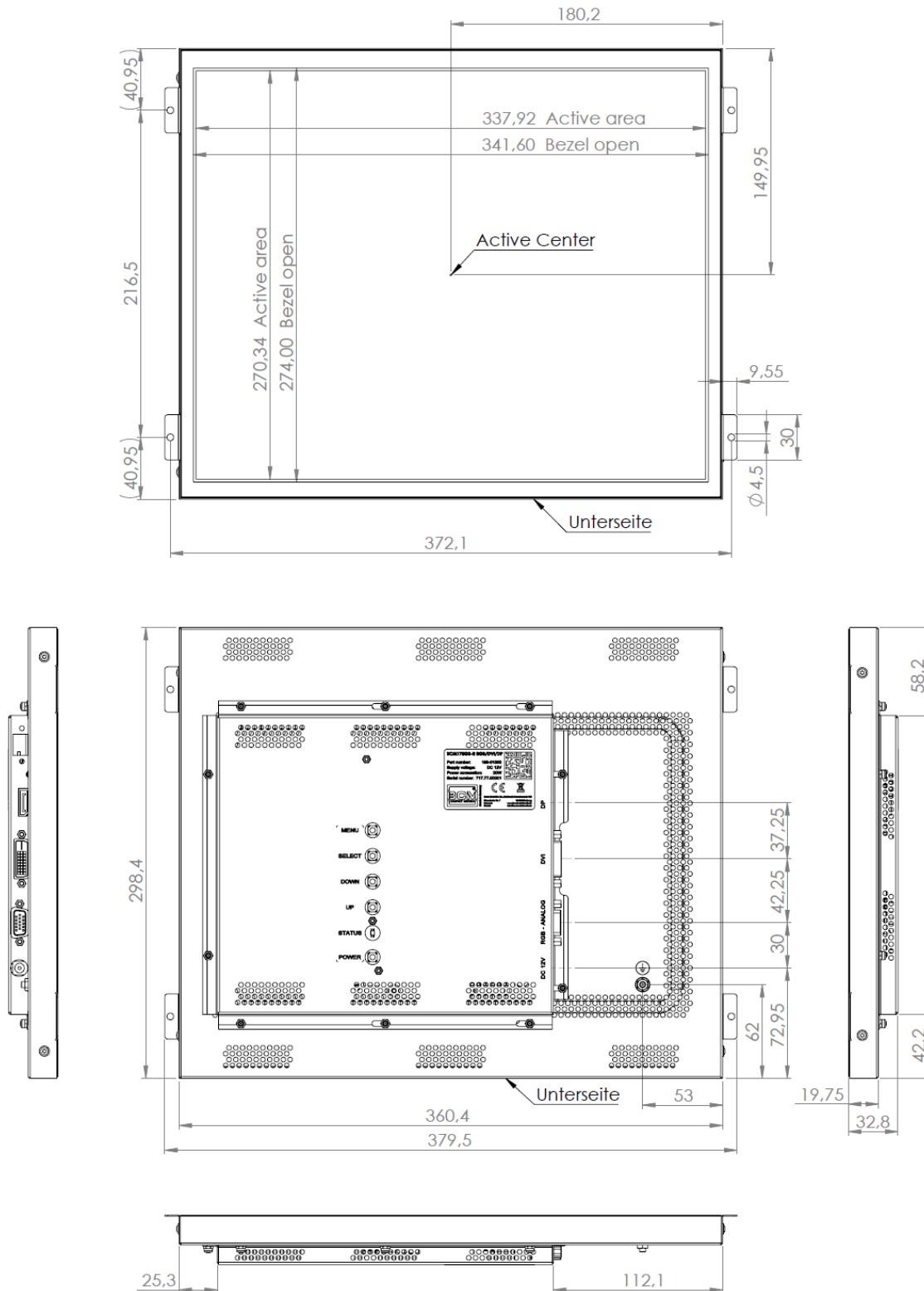
Figure 1: Mechanical Outlines
