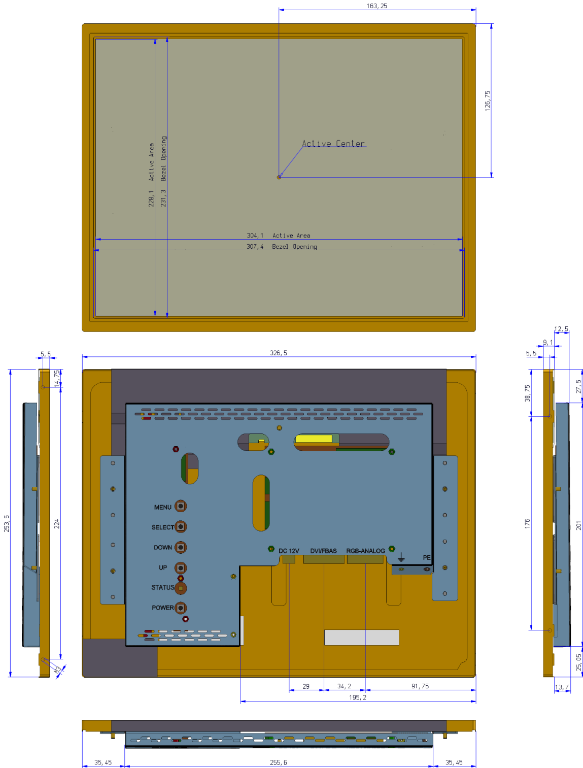
Figure 1: Mechanical Outlines
