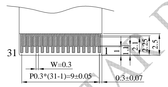
FPC Contact Side SCALE 1:2.5
