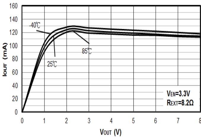
Figure 12. V_{OUT} vs. I_{OUT} ( R_{EXT}=8.2\Omega )
