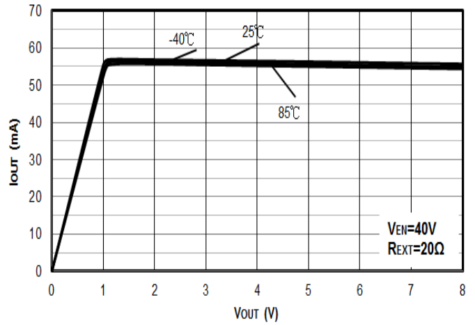
Figure 2. V_{OUT} vs. I_{OUT} ( R_{EXT}=20\Omega )
