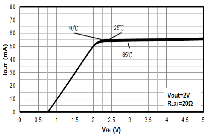
Figure 14. V_{EN} vs. I_{OUT} ( R_{EXT}=20\Omega )
